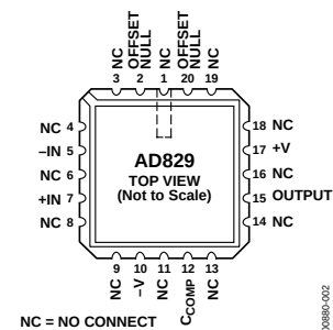
Figure 2. 20-Terminal LCC
