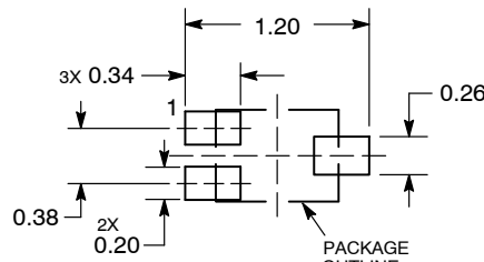
SOLDERING FOOTPRINT*
