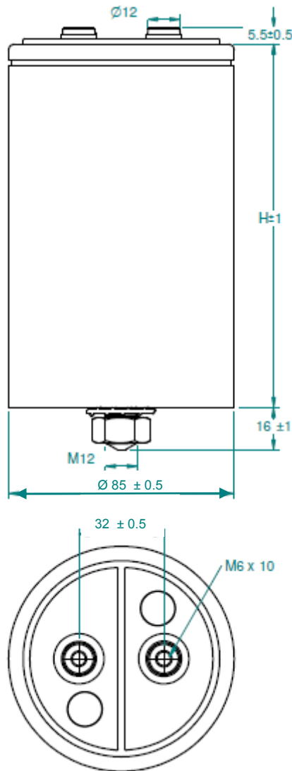
Figure 1: - B25620B - Ø 85mm - Female terminals (M6) - Between terminals 32 \pm 0.5 mm
