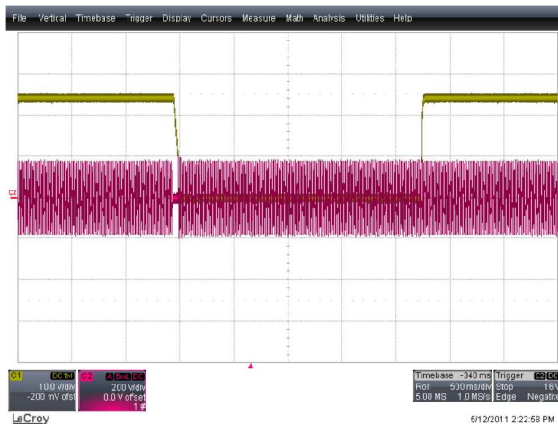
CH1:Vo (10 V/div) CH2:Vin (200 V/div) Figure 11: AC drop out 50 mS@115 VAC (50 mS/div), Vo restart
