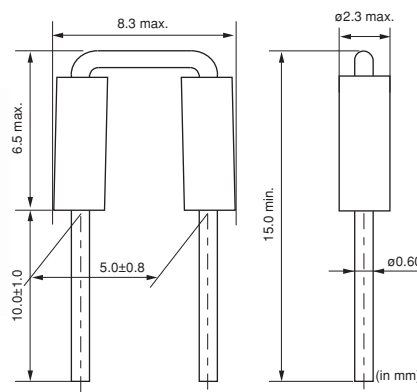
BL03RN2R1M1B
