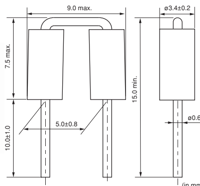
BL02RN2R1M2B
