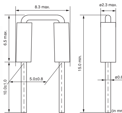
BL03RN2R1M1B
