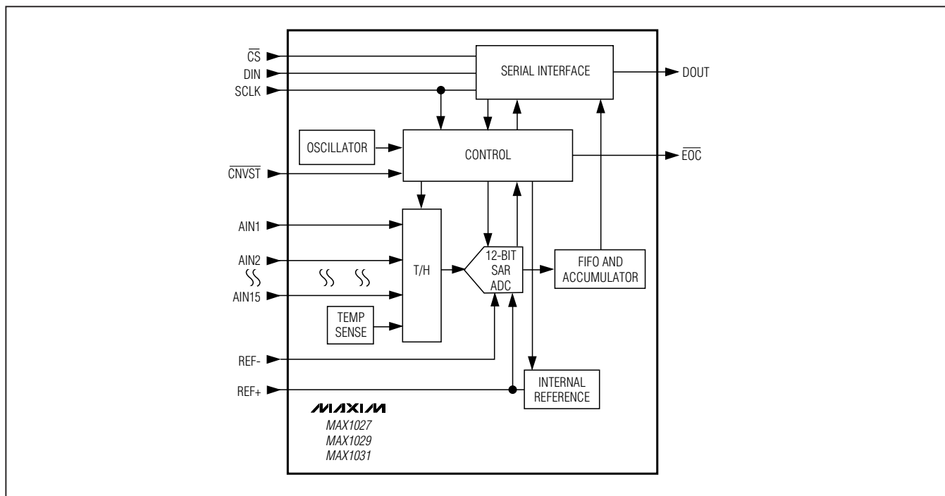
Figure 2. Functional Diagram
