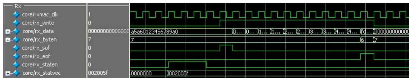
Figure 2-8. Reception of a 64 Data Byte Frame
