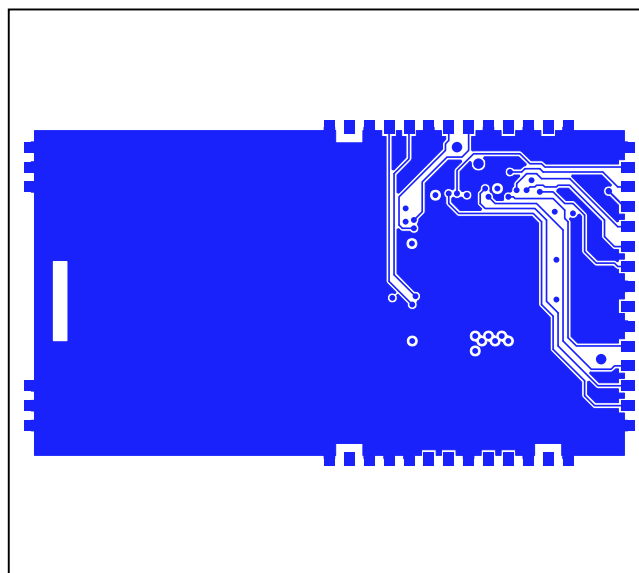
SC1905-DB1900—PCB Layout—Bottom
