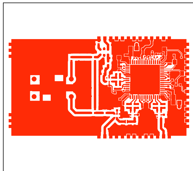
SC1905-DB1900—PCB Layout—Top
