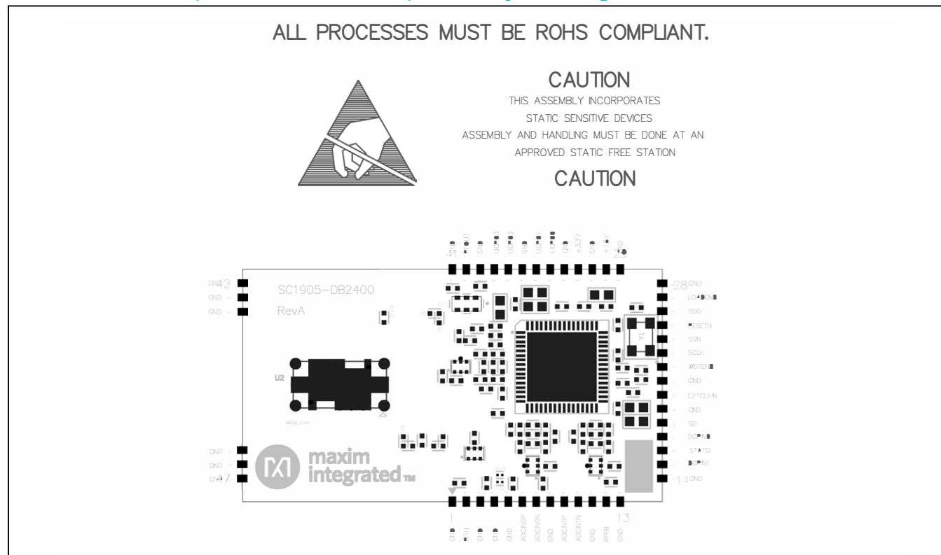
SC1905-DB2400—Assembly Drawing
