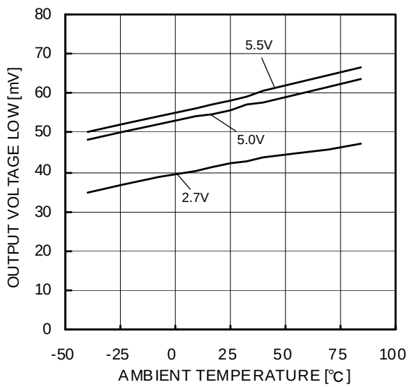
Figure 8. Maximum Output Voltage(Low) – Ambient Temperature ( R_L=2k\Omega )
