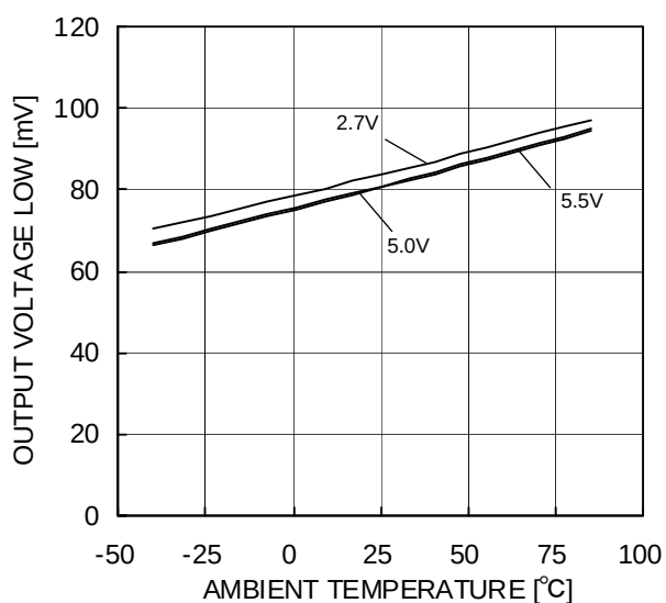
Figure 56. Maximum Output Voltage(Low) – Ambient Temperature ( R_L=2k\Omega )
