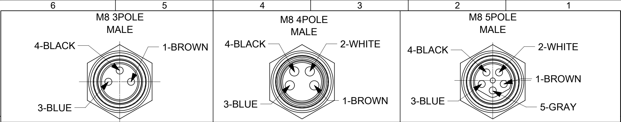
VIEWS FROM THE FRONT SIDE
