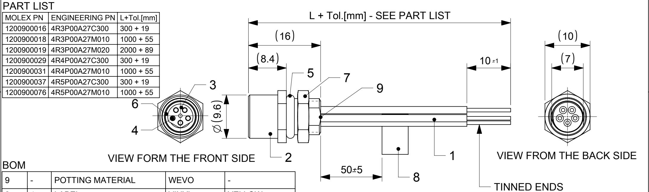
VIEWS FROM THE FRONT SIDE
