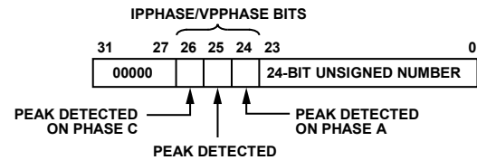
Figure 60. Composition of IPEAK[31:0] and VPEAK[31:0] Registers
