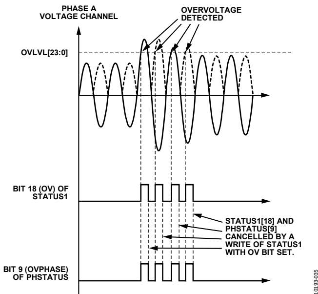
Figure 62. Overvoltage Detection
