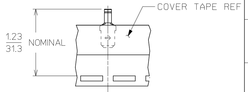
TAPE MOUNTING LOCATION FOR I90220010, AMCT-1T
