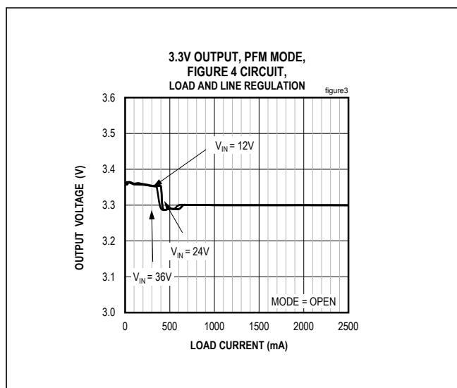
Figure 3. MAX17543 3.3V Output Load and Line Regulation (PFM Mode)
