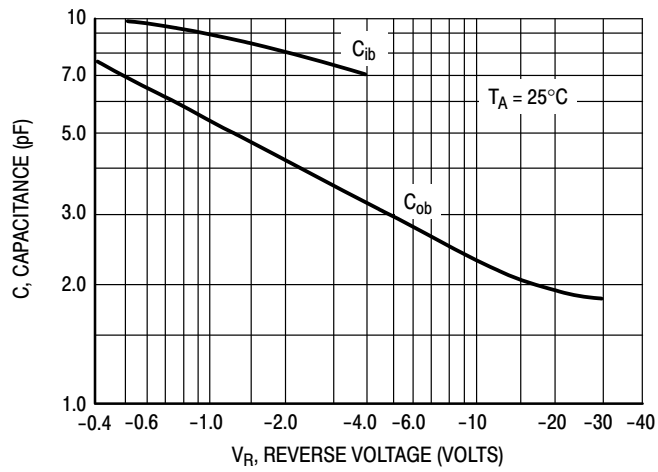
Figure 47. Capacitances
