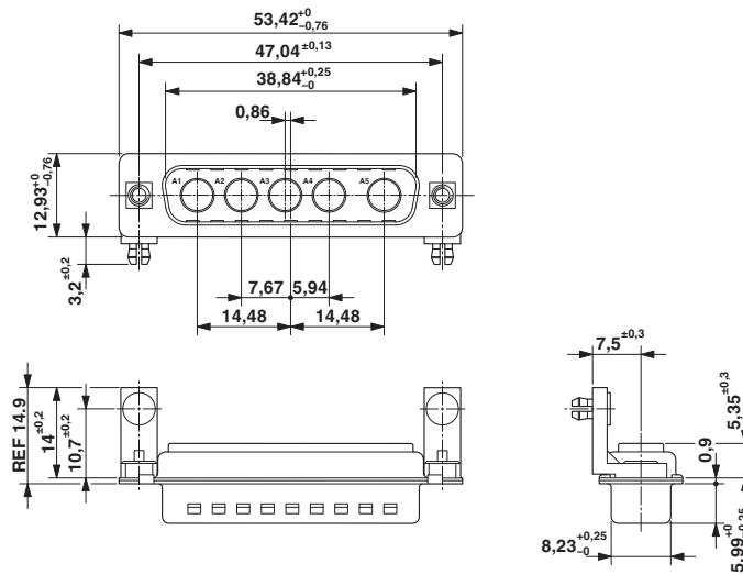
Dimensioned drawing
