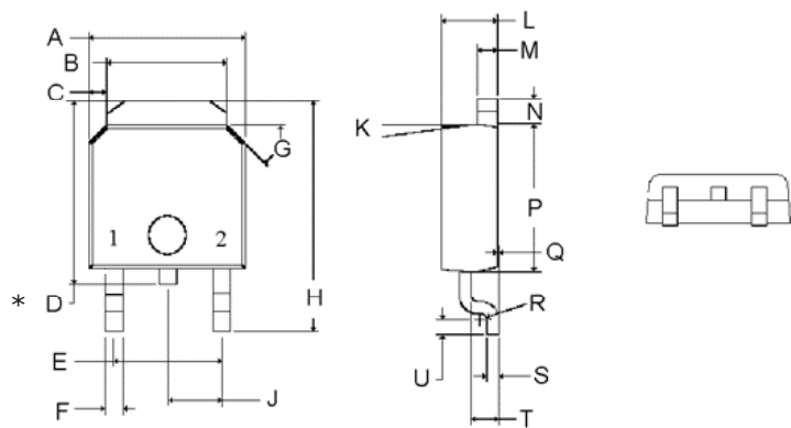
Package TO-252-2
