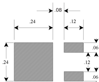
TO-252-2
