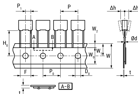
Figure 2 – Lead Spacing 7.5 mm
