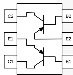
Figure 4. FMB2907A Internal Connections
