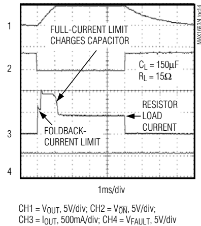
MAX1693 STARTUP TIME (TYPICAL USB APPLICATION)
