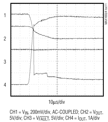
MAX1693 CURRENT-LIMIT RESPONSE
