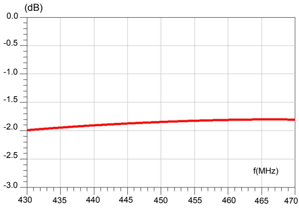
Figure 1. Insertion loss
