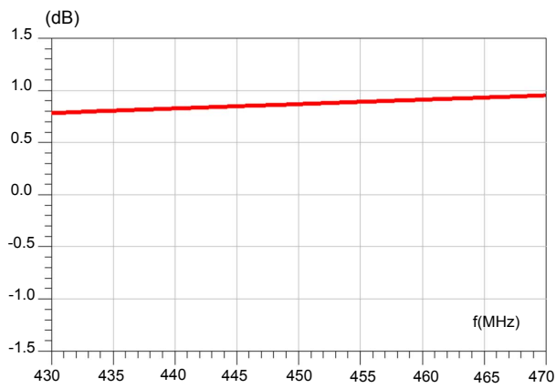
Figure 3. Amplitude imbalance
