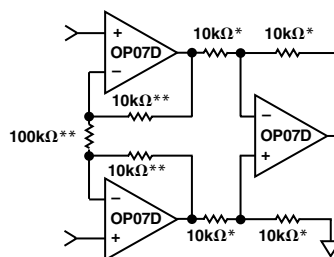
3 OP AMP, IN AMP, G = 100 * 0.02% RESISTOR MATCH, 3PPM/°C TRACKING ** DISCRETE 1% RESISTOR, 100PPM/°C TRACKING SUPPLY CURRENT = 15mA MAX
