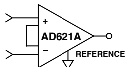
AD621A MONOLITHIC INSTRUMENTATION AMPLIFIER, G = 100 SUPPLY CURRENT = 1.3mA MAX
