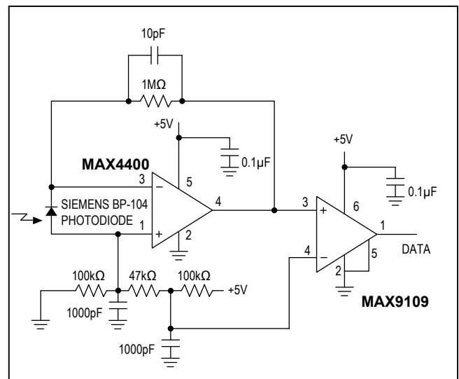
Figure 4. Battery-Operated Infrared Data Link Consumes Only 760μA
