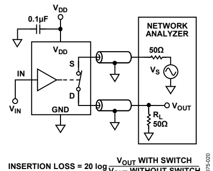
Figure 20. Bandwidth
