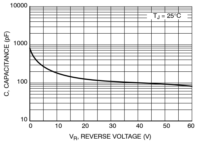
Figure 10. Capacitance
