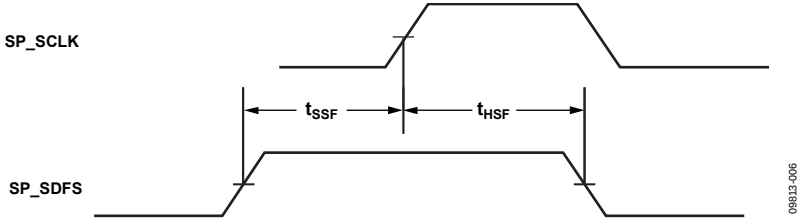
Figure 6. Slave Mode SP_SDFS Setup/Hold Time
