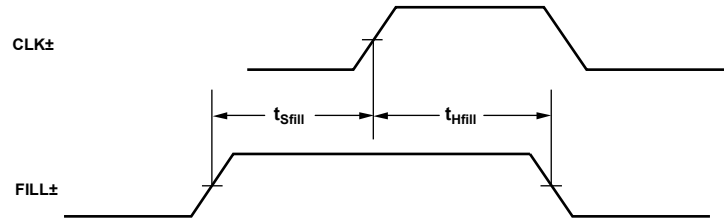
Figure 7. FILL± Setup and Hold Times
