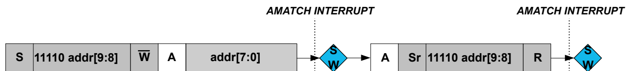
Figure 34-11. 10-bit Addressing
