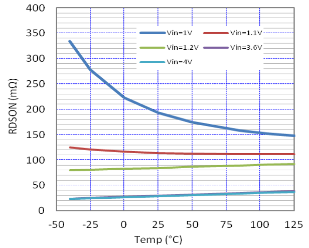
Figure 7. R_{DS(on)} (mΩ) vs. Temperature (°C)
