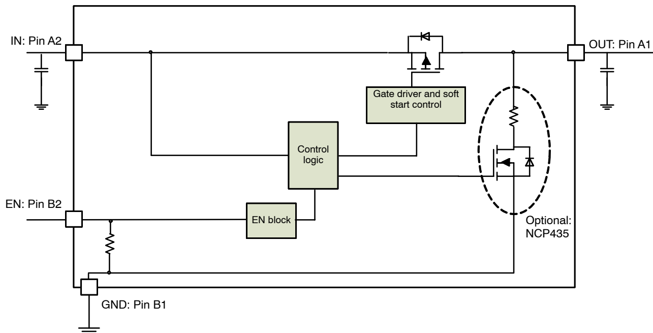
Figure 2. Block Diagram
