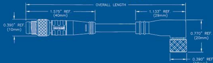
STRAIGHT/90° MALE/FEMALE DOUBLE ENDED THREADED COUPLING
