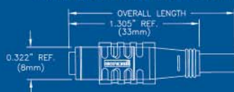
STRAIGHT MALE SINGLE ENDED SNAP LOCK
