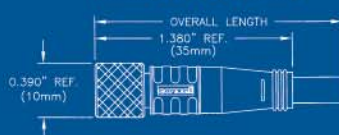
STRAIGHT FEMALE SINGLE ENDED THREADED COUPLING
