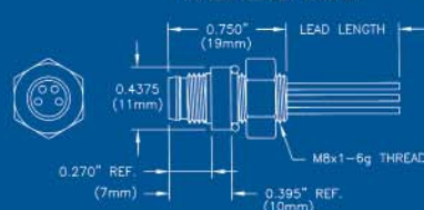
MALE RECEPTACLE
