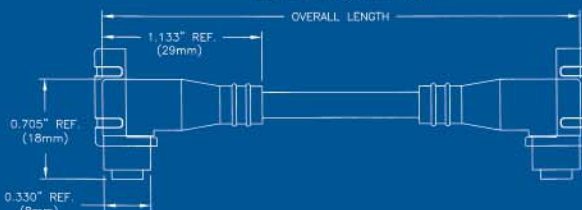
FEMALE RECEPTACLE
