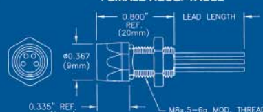
FEMALE RECEPTACLE
