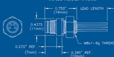
MALE RECEPTACLE
