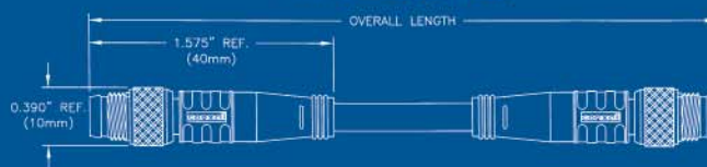
STRAIGHT/90° MALE/FEMALE DOUBLE ENDED THREADED COUPLING
