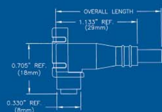
90° FEMALE SINGLE ENDED SNAP LOCK WITH LOCKING RING
