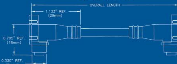
FEMALE RECEPTACLE
