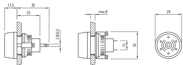
04 Buzzer Raised
