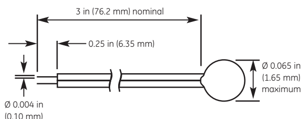
NTC Interchangeable Type MC65 dimensions
