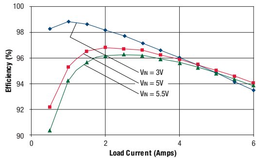
Efficiency vs. Line Voltage and Load Current @ +25°C ( V_{OUT} = 2.5V )
