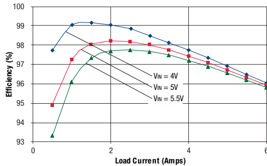
Efficiency vs. Line Voltage and Load Current @ +25°C (V out = 3.3V)
