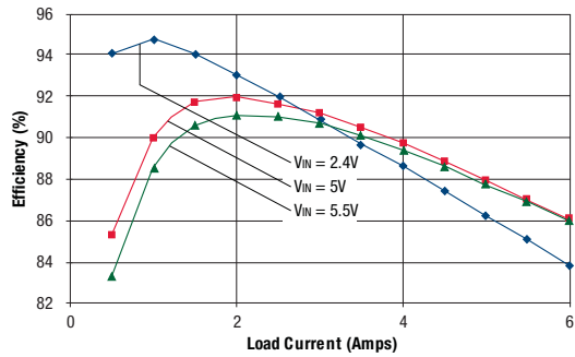
Efficiency vs. Line Voltage and Load Current @ +25°C ( V_{OUT} = 1.2V )
