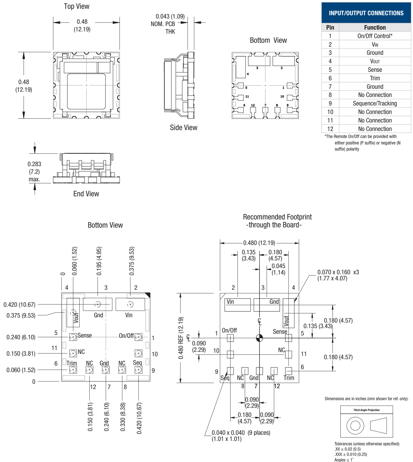
Figure 3. OKL-T/6-W5 Mechanical Outline
