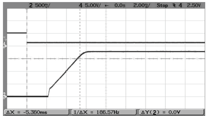
On/Off Enable Startup ( V_{IN} = 5V , V_{OUT} = 1.8V , I_{OUT} = 6A , C_{LOAD} = 0 ) Trace 4=Enable, Trace2=Vout
