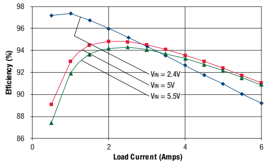
Efficiency vs. Line Voltage and Load Current @ +25°C ( V_{OUT} = 1.8V )
