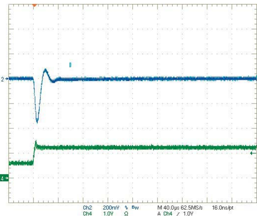
Step Load Transient Response ( V_{IN} = 5V , V_{OUT} = 1.2V , I_{OUT} = 3A to 6A) Trace 2=Vout, 200 mV/div. Trace 4=Iout, 5A/div.
