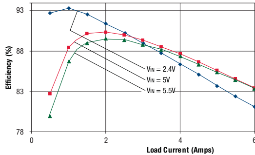
Efficiency vs. Line Voltage and Load Current @ +25°C ( V_{OUT} = 1.0V )
