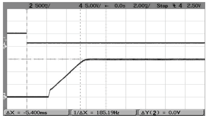
On/Off Enable Startup ( V_{IN} = 5V , V_{OUT} = 1.5V , I_{OUT} = 6A , C_{LOAD} = 0 ) Trace 4=Enable, Trace2=Vout
