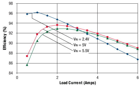
Efficiency vs. Line Voltage and Load Current @ +25°C ( V_{OUT} = 1.5V )
