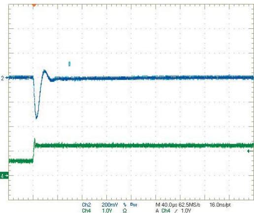
Step Load Transient Response ( V_{IN} = 5V , V_{OUT} = 1.8V , I_{OUT} = 3A to 6A) Trace 2=Vout, 200 mV/div. Trace 4=Iout, 5A/div.
