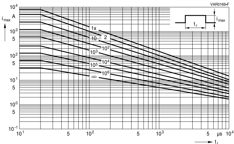
SIOV-S20K385 ... K460
