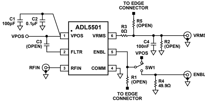
Figure 56. Evaluation Board Schematic
