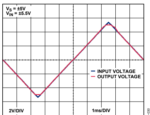
Figure 30. No Phase Reversal
