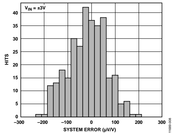
Figure 8. Typical Distribution of System Error
