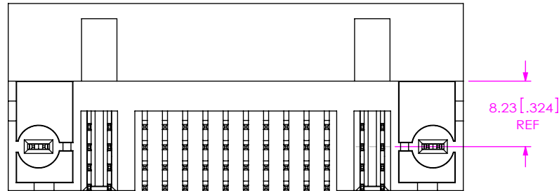
FIG 2 PETC-01-40-01-X-RA-LC SHOWN (SAME AS FIG 1, UNLESS OTHERWISE STATED)
