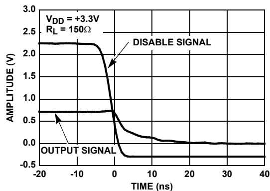
FIGURE 14. DISABLE TIME
