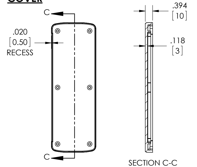
DIE CAST ALUMINUM COVER
