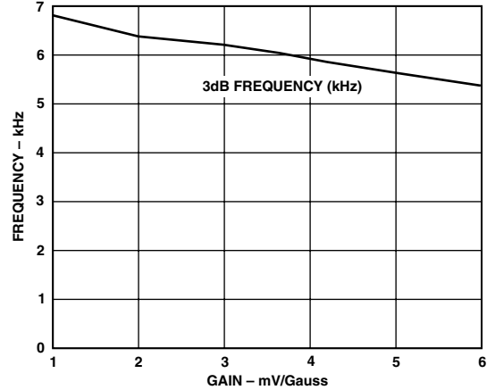
Figure 13. Small Signal Gain Bandwidth vs. Gain
