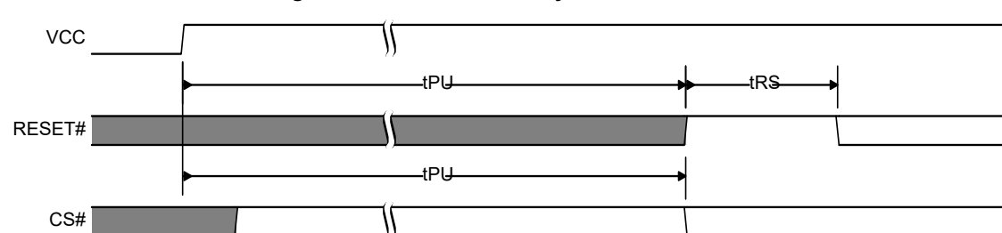
Figure 138. POR followed by Hardware Reset
