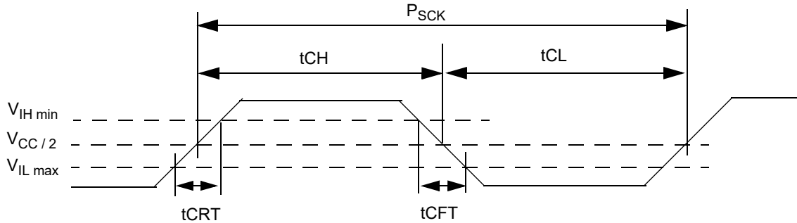
Figure 142. Clock Timing
