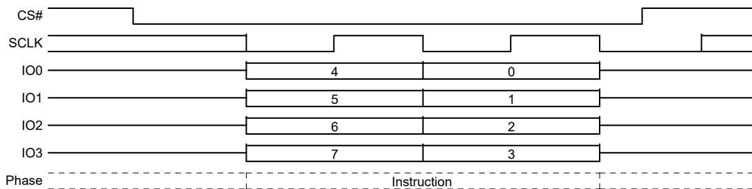
Figure 90. Program or Erase Suspend Command with Continuing Instruction Commands Sequence
