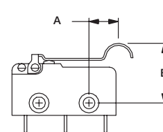
FIG. 6 Simulated Roller
