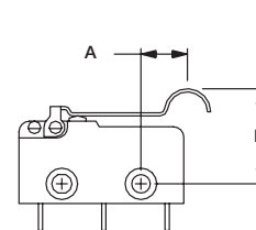
FIG. 6 Simulated Roller
